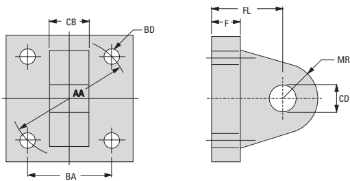
Eye Bracket
