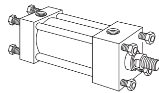
IHML Both ends extended tie rod ISO MX1
